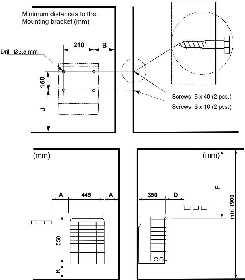
Image 2 Safety clearances
