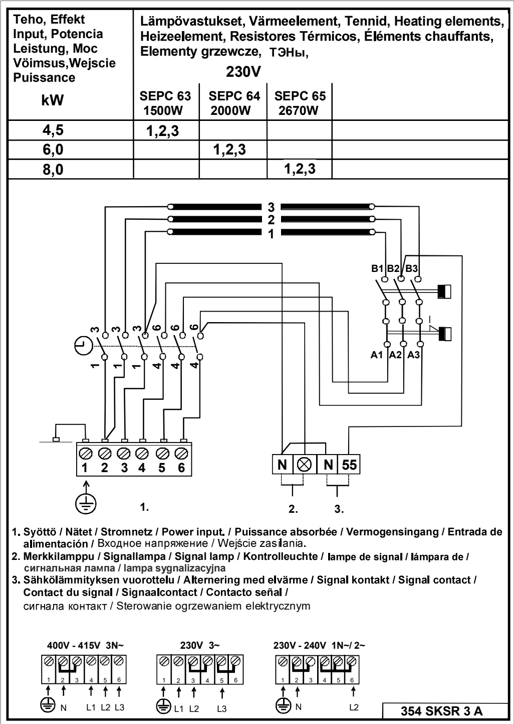
Image 4 Switch diagram for the sauna heater
